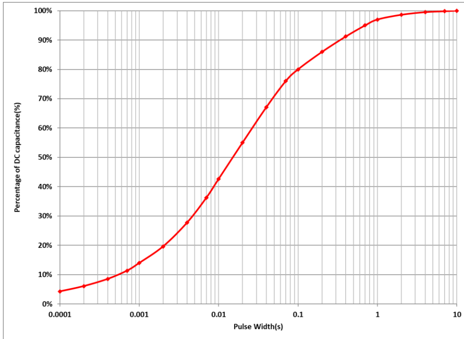
Figure 4: Effective Capacitance
