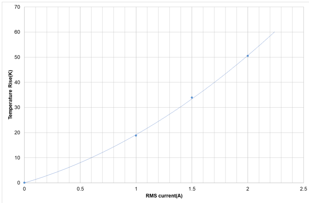
Fig 12: Temperature rise in DMHA14R5V353M4ATA0 with RMS current
