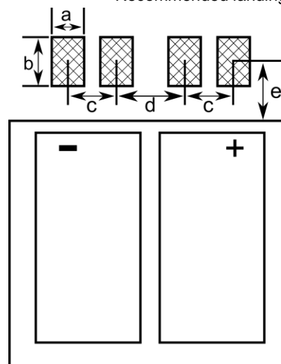
Recommended landing pads
