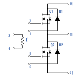
Half Bridge with Recovery Diode (3x6A)
