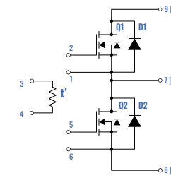
Half Bridge with Recovery Diode (3x6B)
