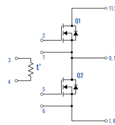
Half Bridge (6x6)
